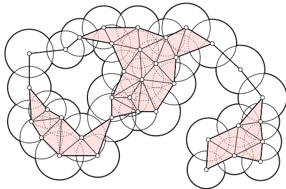
Figure 4: A finite set of disks and the canonical realization of an abstract simplicial complex over that set. The vertices, edges, and triangles correspond to abstract simplices of dimension 0, 1, and 2. Take a moment to verify that all simplices are independent.
