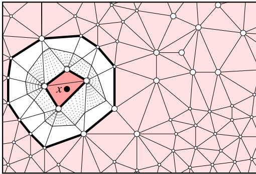
Figure 7: The point x is contained in four disks, which induce the dark-gray subcomplex \bar{K}_x , consisting of two triangles and their faces. The other disks induce the light-gray subcomplex \bar{L}_x . We get \bar{Z}_x by adding initial portions of the line segments covering the white in-between simplices to the underlying space of \bar{K}_x .
